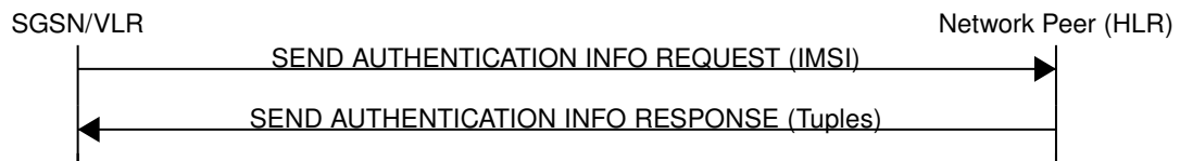
Figure 13: Send Authentication Info (Normal Case)
