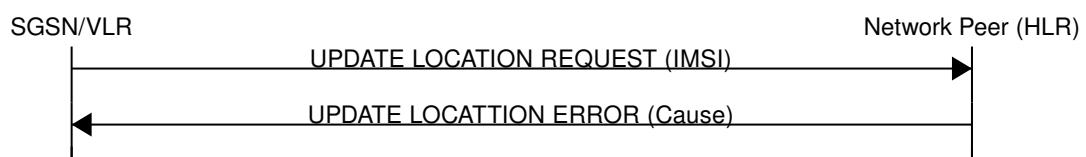
Figure 17: Update Location (Error Case)
