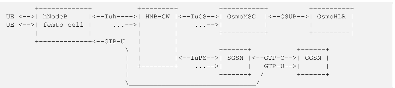
Typical 3G network architecture used with OsmoHNBGW
